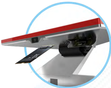
Removable SSD
